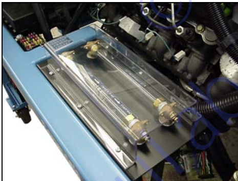
EM-514, A/C SYSTEM WITH SIGHT GLASSES
